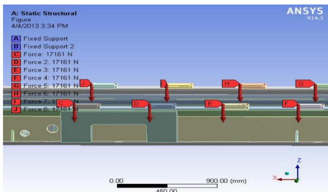
Fig 4: Load Application
