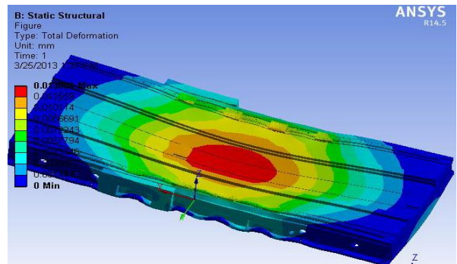
Fig 5: Total Deformation of BED 1.0
