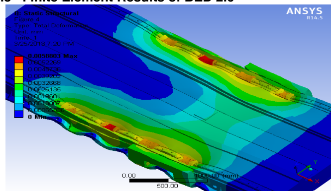
Fig 7: Total Deformation of BED 2.0
