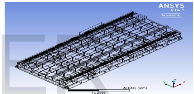
Fig 3: Geometry of BED 3.0 (wire mesh view)
